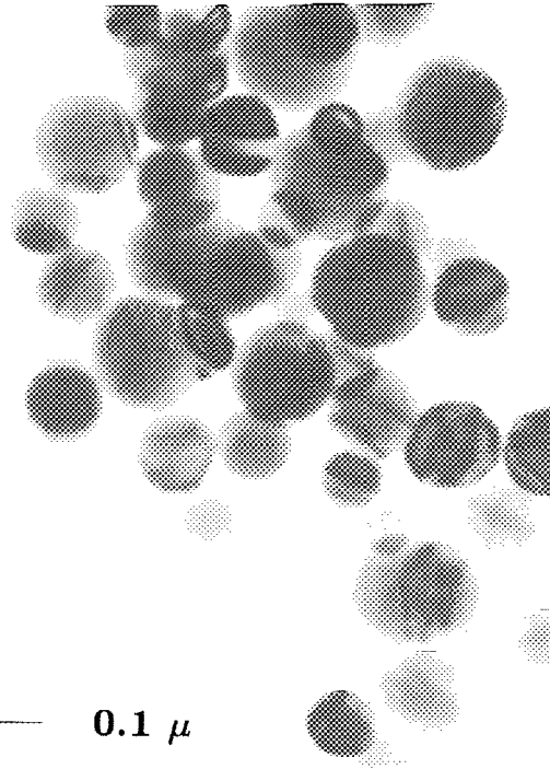
FIG. 4. TEM photographs of the crystalline silicon particles that accounted for about 99% of the particles produced by rate controlled thermal decomposition of silane.
