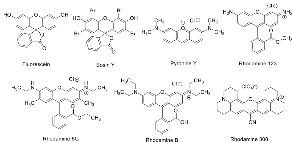
Figure 14. Common xanthone and xanthylum fluorescent dyes used for luminescent detection applications 502-543
