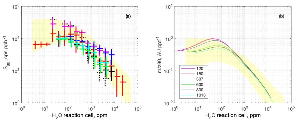
Figure 6. Same as Fig. 5 except for \text{O}_2^- (\text{CH}_3\text{OOH}) .
