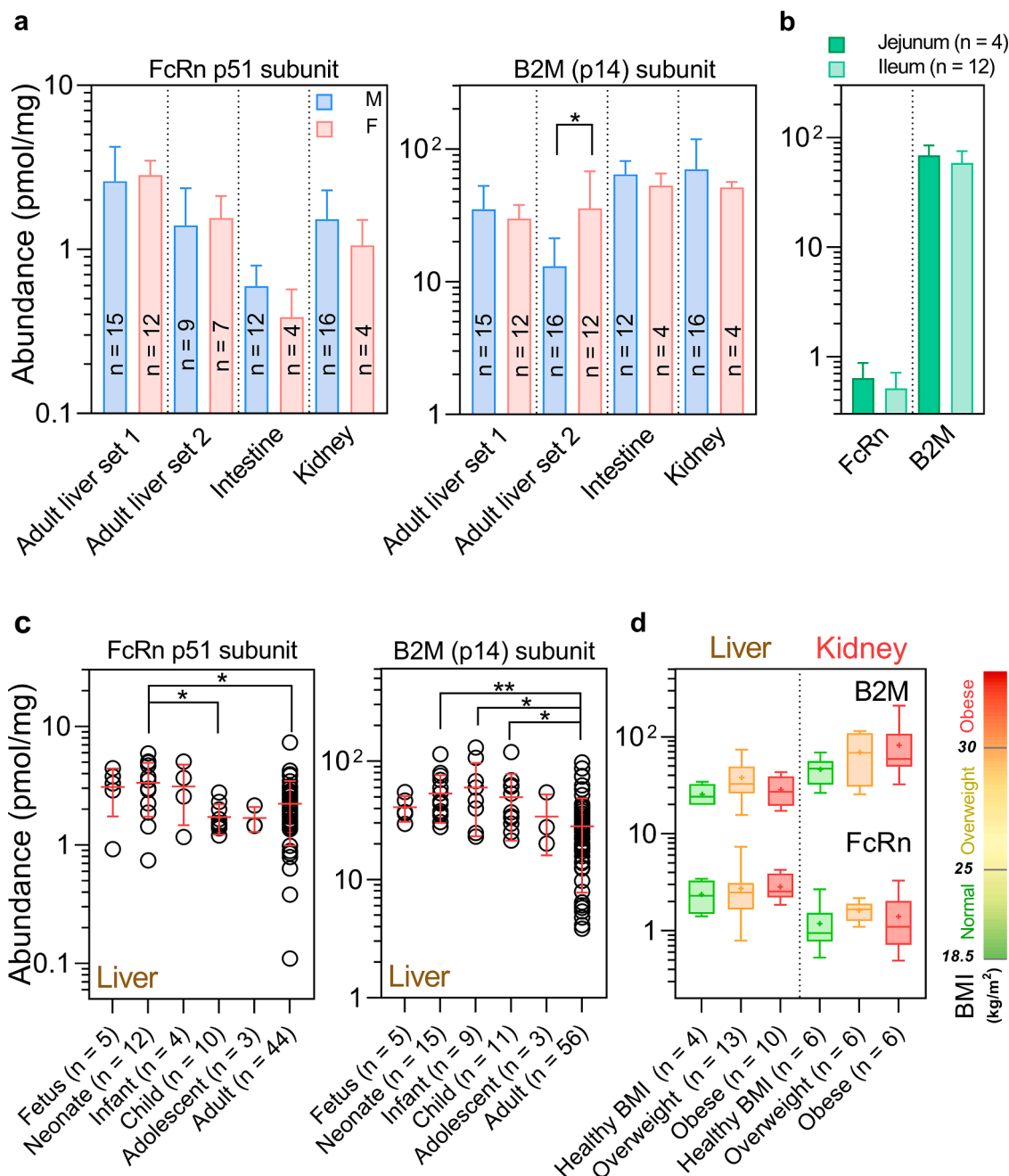
Fig. 2. Covariates of protein expression of FcRn subunits p51 and B2M in three tissues. The variables assessed are sex (a), intestinal anatomical region (b) and age (c) and body mass index, BMI (d). Sex did not affect the expression of FcRn in liver, intestine and kidney (a). There were no differences in FcRn abundance between jejunum and ileum (b). Binning expression data into developmental age groups [EMA categories: fetal, neonates (0–1 month), infants (>1 month–23 months), children (2 years–11 years), adolescents (12 years–17 years), adults (18 years and over)] showed an ontogeny-related decline in FcRn abundance with age until adulthood (c). An overall rise in abundance of FcRn p51 and B2M proteins in liver and kidney was observed with increasing BMI (d). Units of abundance are pmol per mg membrane protein (liver and kidney), pmol per mg mucosal protein (intestine) or pmol per mg post-mitochondrial supernatant protein (skin). In panels a, b and c, abundance data are presented as means and error bars represent standard deviation (SD) values. In panel a, M, male; F, female; * p < 0.05 ( t -test). In panel d, the whiskers reflect the ranges, the boxes reflect the 25th and 75th percentiles, the lines are the medians, and the + signs are the means. The scale inset represents BMI categories (normal BMI: 18.5 – 25, overweight: 25–30, obese: >30 kg/m 2 ). In panel c, p -value cut-offs were Bonferroni-corrected in post-hoc tests to: * p < 0.01 ; ** p < 0.002 .
