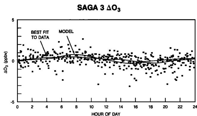
Fig. 6. Diurnal behavior of O_3 on SAGA 3 from measurements by the NOAA/PMEL instrument. The best fit to data and model-computed diurnal behavior of O_3 , (O_3(t) - \text{diurnally averaged } O_3) calculated at 1-hour intervals, are also shown.
