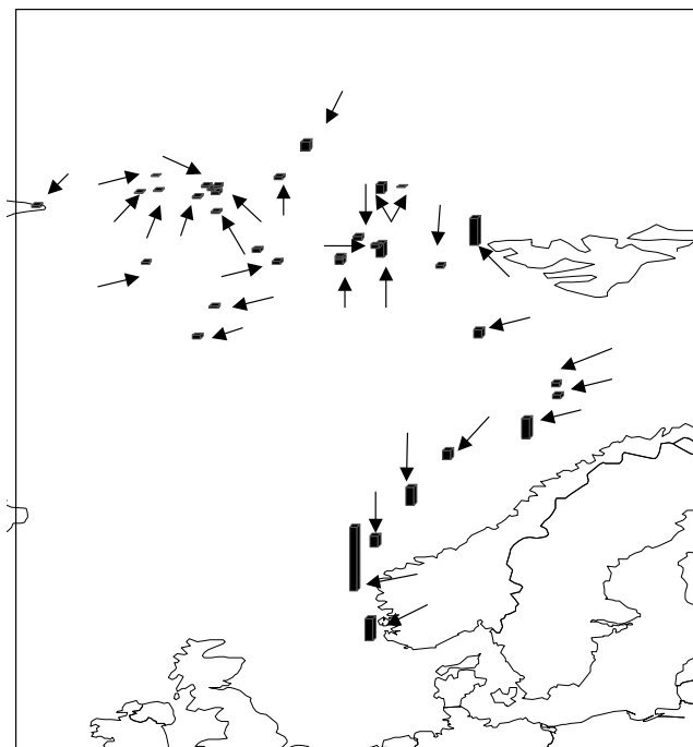
Figure 2. Spatial distribution of \Sigma_{\text{ICES}} polychlorinated biphenyl (PCB) in air along the cruise ( n = 37 ). Note that the bars center on the average sample location. Largest bar is 100 \text{pg m}^{-3} (site 2); smallest bar is 0.76 \text{pg m}^{-3} (site 31). Black arrows indicate general recent direction of the 72 h back trajectories for each sample.
