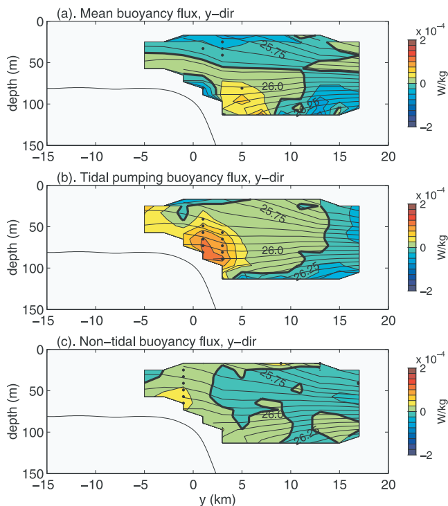
Figure 6. Computed cross-isobath buoyancy fluxes. (a) Mean flux ( \overline{v'b} ). (b) Tidal pumping flux ( \overline{(\overline{v'})'(\overline{b'})'} ). (c) Nontidal flux ( \overline{(\overline{v'})'(\overline{b'})'} ). Zero flux contours are drawn as heavy black lines and the mean density field is shown by the thin black lines. The black dots show the locations where the computed flux is significantly different from zero at the 95% level.
