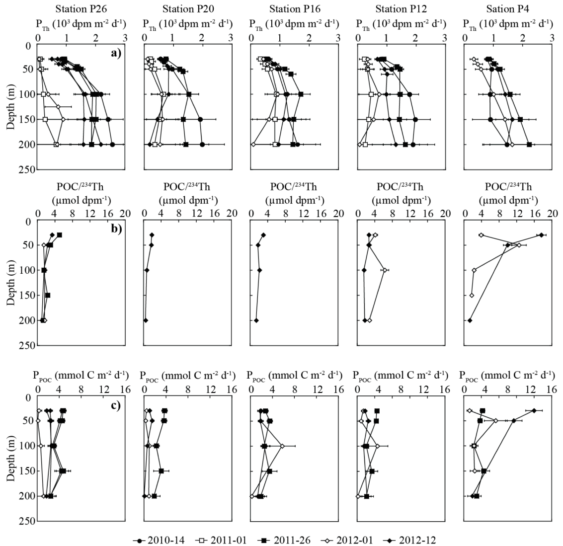
Figure 9. Depth profiles of a) ^{234}\text{Th} fluxes ( P_{Th} ) determined using the 2-D model, b) POC/ ^{234}\text{Th} ratios on >53 \mu\text{m} particles, and c) ^{234}\text{Th} -derived POC fluxes ( P_{POC} ) at stations on Line P during the five cruises in this study.
