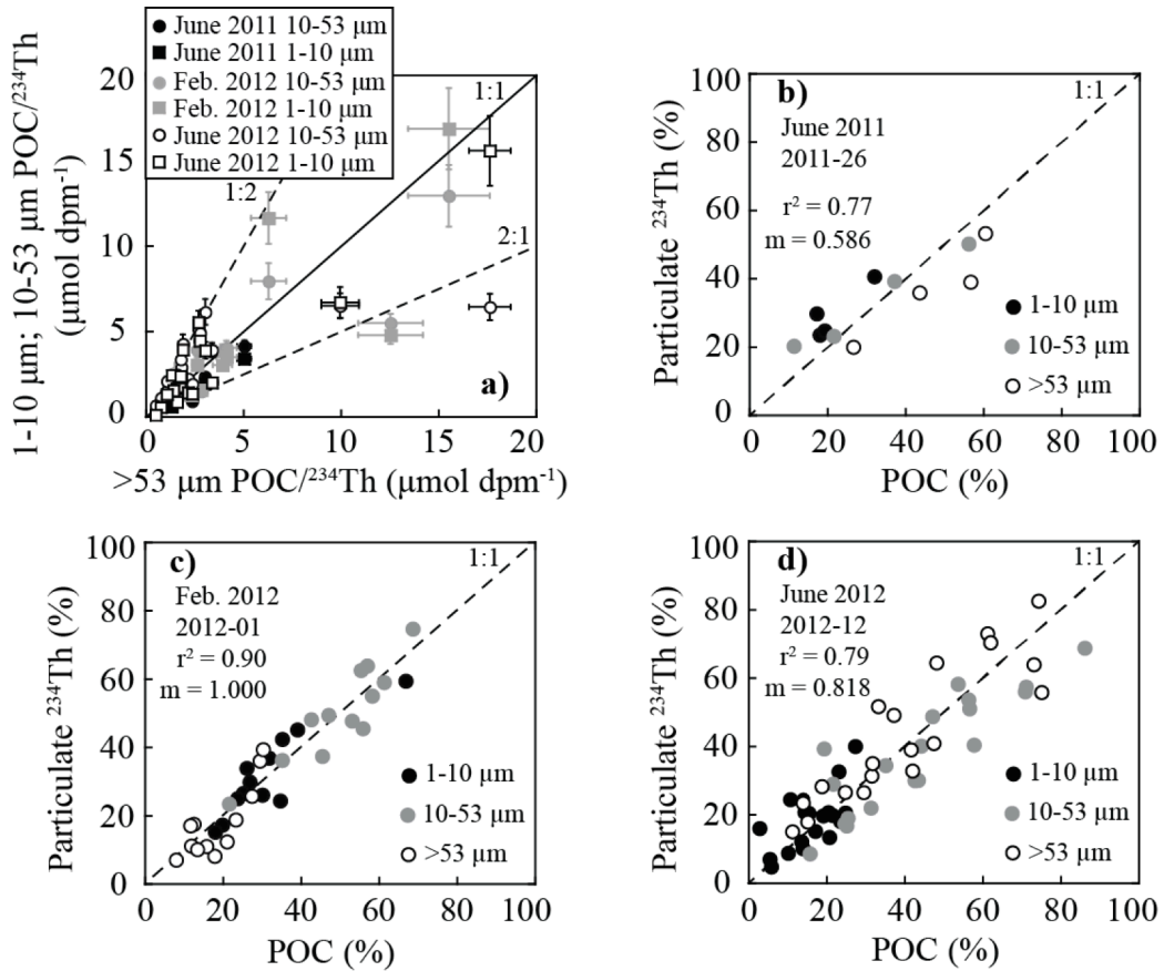
Figure 4. a) POC/ ^{234}\text{Th} ratios on 1 – 10- \mu\text{m} particles and on 10 – 53- \mu\text{m} particles plotted against the POC/ ^{234}\text{Th} ratio on >53- \mu\text{m} particles. Fractional distributions of POC and particulate ^{234}\text{Th} are plotted for three size-classes of particles. The percentage of total POC associated with each particle size-class is plotted against the percentage of total particulate ^{234}\text{Th} for samples collected at stations on Line P during b) June 2011, c) February 2012, and d) June 2012. The correlation coefficient ( r^2 ) and the slope of the linear regression ( m ) are shown for each cruise.
