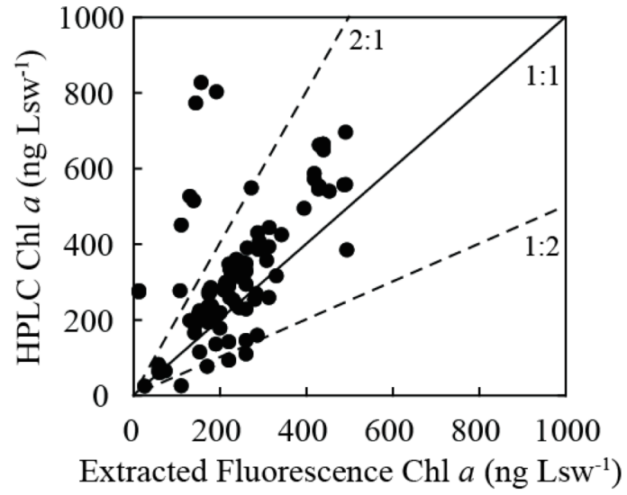
Figure A1. Comparison of fluorescence and high-performance liquid chromatography (HPLC) measurements of Chl a concentrations.
