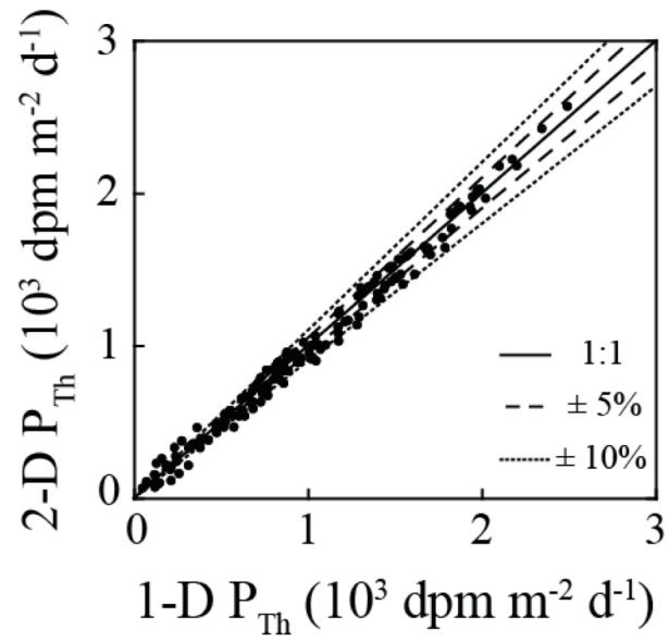
Figure A4. ^{234}\text{Th} fluxes determined by the 1-D steady-state model compared to those determined by the 2-D steady-state model. Dashed and dotted lines envelope 5% and 10% error ranges respectively.
