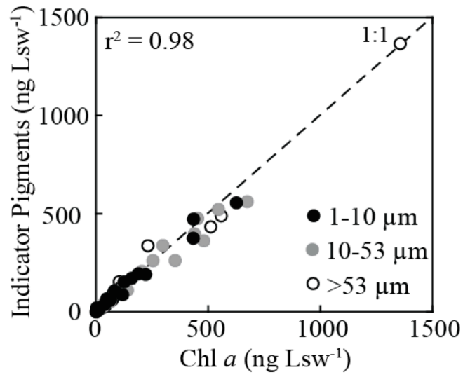
Figure A3. Chl a concentrations plotted against total indicator pigment concentrations for three size-fractions of particles collected by in-situ pumps. The correlation coefficient ( r^2 ) is also shown.
