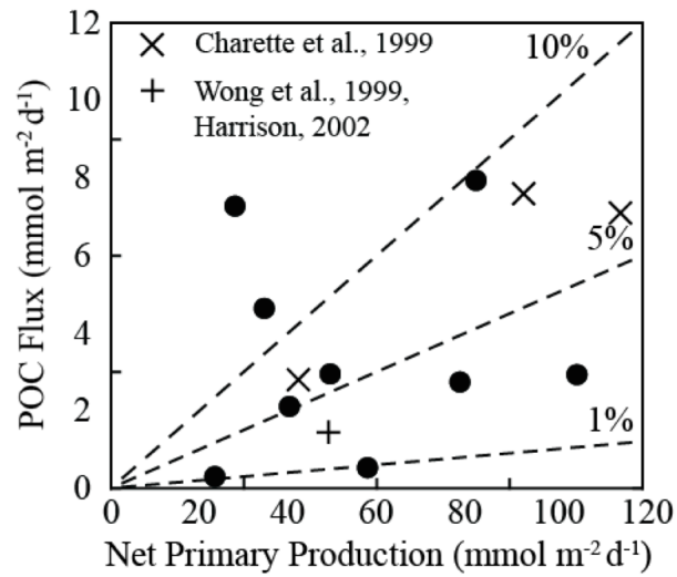
Figure 10. Net primary production (NPP) plotted against ^{234}\text{Th} -derived POC fluxes ( P_{\text{POC}} ) for stations along Line P in this study. The slopes of the dashed lines represent ThE -ratios. For reference NPP and P_{\text{POC}} values determined by Charette et al. (1999) for winter, spring and summer are included, along with annual average NPP and sediment trap POC fluxes (at 200 m) reported in Harrison (2002) and Wong et al. (1999) respectively.
