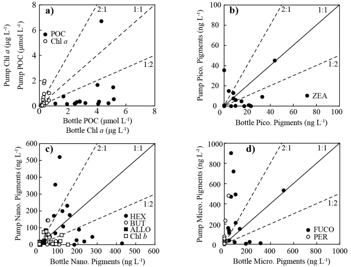
Figure 3. Comparison of small-volume Niskin bottle and large-volume in situ pump measurements of a) POC, b) picoplankton indicator pigments, c) nanoplankton indicator pigments, d) microplankton pigments. Niskin bottle measurements are lower than pump measurements for microplankton pigments, and higher for nanoplankton pigments and POC.
