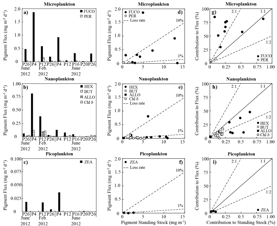
Figure 12. a-c) ^{234}\text{Th} -derived indicator pigment fluxes determined using the Pigment/ ^{234}\text{Th} ratio on >53\text{-}\mu\text{m} particles plotted for micro-, nano-, and picoplankton pigments. d-f) Indicator pigment standing stocks plotted against indicator pigment fluxes for micro-, nano-, and picoplankton pigments. The slopes of the dashed lines indicate pigment loss rates. g-i) The contribution to total pigment standing stock plotted against the contribution to total pigment flux for micro-, nano-, and picoplankton pigments. Data points above the 1:1 line indicate preferential export by direct sinking and points below the 1:1 line indicate disproportionately low export by direct sinking relative to biomass contributions.
