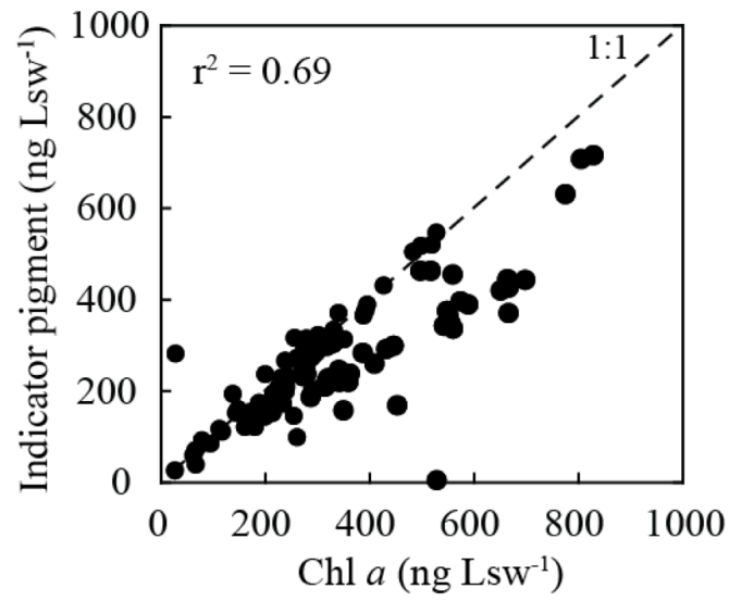
Figure A2. Chl a concentrations plotted against total indicator pigment concentrations for Niskin bottle samples. The correlation coefficient ( r^2 ) is also shown.
