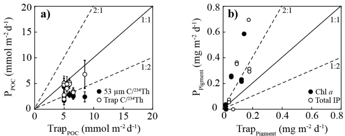
Figure 11. a) Comparison of sediment trap POC fluxes and ^{234}\text{Th} -derived POC fluxes, and b) a comparison of sediment trap Chl a and total indicator pigment fluxes and ^{234}\text{Th} -derived pigments fluxes at OSP during June 2011 and June 2012.
