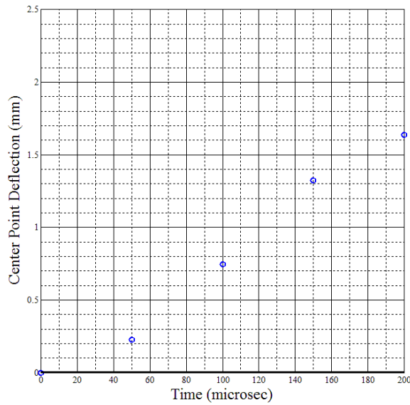
Figure 3.2.7.1-1: Outward center point deflection, WWHT experiment 1
