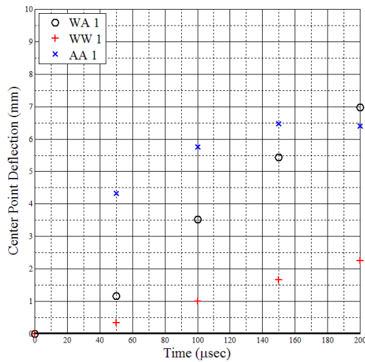
Figure 4.2.1-4: Abbreviated deflection plot of the WA 1, WW 1, and AA 1 experiments, up to 200 μsec.
