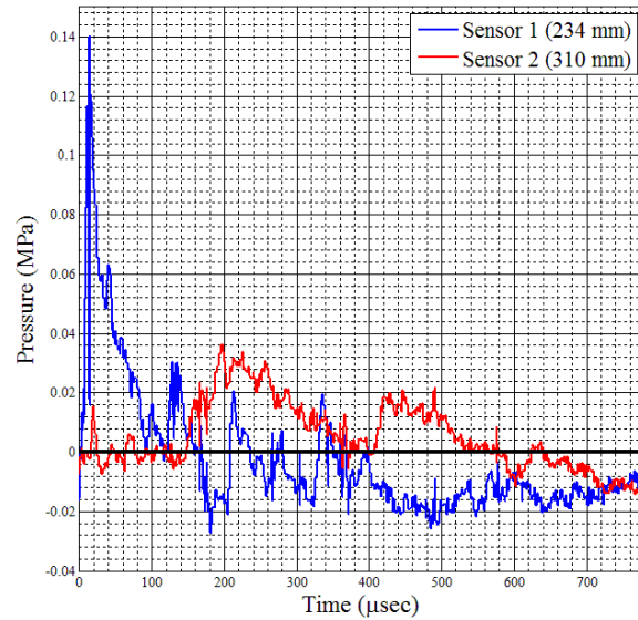
Figure 3.2.3.4-1: Filtered plot of pressure data collected during AA experiment 4.
