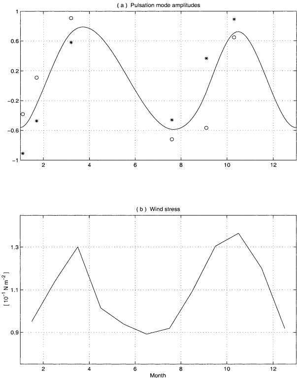
FIG. 15. (a) The pulsation mode amplitudes for salinity in the layer 0–300 dbar (star) and for salinity in the layer 300–3000 dbar (circle). The curve is a smoothing spline fit to the data repeated for three years and displayed for the central year. (b) The averaged eastward wind stress within a square of 120°–160°E and 45°–60°S, based on Southampton Oceanography Centre Global Air–Sea Heat and Momentum Flux Climatology (GASC97) surface climatological data.
