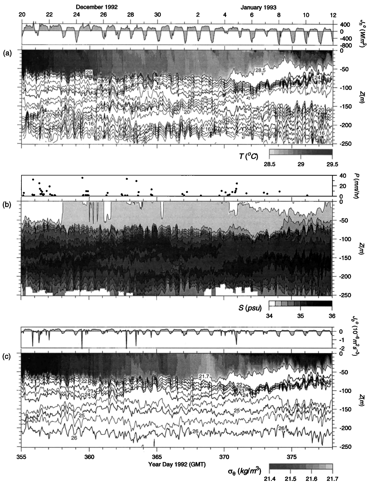
Figure 3. (a) Temperature. Values above 28.5 ^{\circ}\text{C} are shaded at 0.05 ^{\circ}\text{C} intervals. The contour interval is 1 ^{\circ}\text{C} , with an added contour at 28.5 ^{\circ}\text{C} . (b) Salinity. Contour interval is 0.2 practical salinity units (psu). (c) Potential density. Values below 21.7 \text{kg m}^{-3} are shaded at 0.025 \text{kg m}^{-3} intervals. Otherwise, the contour interval is 0.5 \text{kg m}^{-3} . Profiler data were averaged into 1-hour, 4-m bins before contouring. For reference, the hourly surface heat flux, precipitation, and buoyancy flux are included in Figures 3a, 3b, and 3c (top), respectively.
