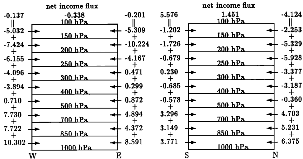
Figure 19. Example of mass flux components across the walls of the box in Figure 16 for September 27, 1991, based on divergent wind calculated from ECMWF data. Units, 10 9 kg s -1 .
