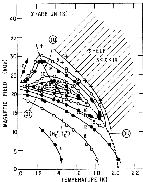
FIG. 4. Contour plot of ac differential susceptibility in the H - T plane for TTF-AuS 4 C 4 (CF 3 ) 4 (solid lines). Ridges in the contours are shown as dashed or dot-dashed lines and correspond to phase boundaries. Values of \chi are in (arbitrary units) such that 1 arb. unit corresponds to 1.89 \times 10^{-4} emu/mole.
