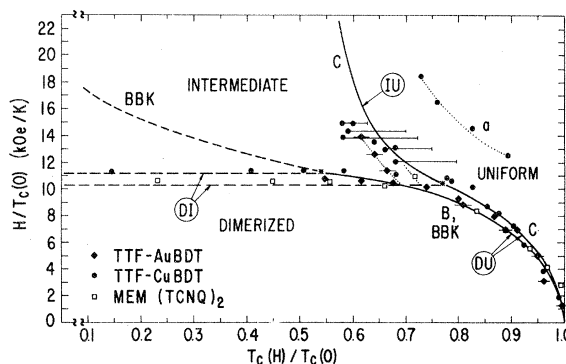
FIG. 9. Composite normalized phase diagram for TTF-AuS 4 C 4 (CF 3 ) 4 , TTF-CuS 4 C 4 (CF 3 ) 4 , and MEM-(TCNQ) 2 powders. The normalized scales are H/T_c(0) and T_c(H)/T_c(0) . Where possible, transitions are located by peak values of (\partial M/\partial T)_H or (\partial M/\partial H)_T (or \chi_{ac} ). For normalization, the values chosen for T_c(0) are 2.03, 10.3, and 18.0 K for the compounds as listed. The line designated (a) represents mean-field estimates for the high-field phase boundary (for Cu) from data using a 10-MW solenoid ( H_{max} = 200 kOe). The solid and dashed lines represent theoretical curves as in Fig. 3.
