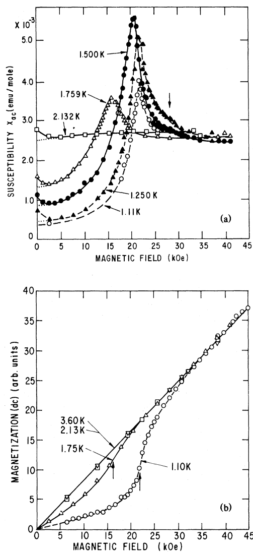
FIG. 2. (a) Differential susceptibility curves at constant temperatures as a function of field. Those curves belonging to the special low-temperature region are shown as dashed lines. At the lowest field, the dotted lines indicate a correction for an impurity effect. The arrow is discussed in Sec. III. (b) Magnetization (static) curves at constant temperatures as a function of field. The arrows indicate the location of \chi_T(H) maxima from (a).
