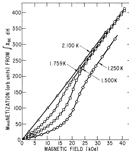
FIG. 7. Field dependence of magnetization as derived by integration of differential susceptibility curves for various temperatures.
