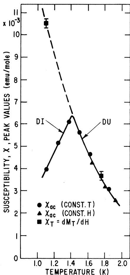
FIG. 8. Magnitude of susceptibility peaks, \chi_{ac} , along the DU and DI phase boundary lines. Also shown are two \chi_{dc} peak points which agree with \chi_{ac} above T_c^* and depart below T_c^* . The discrepancy leaves questions which are difficult to resolve owing to the sparseness of \chi_{dc} data.
