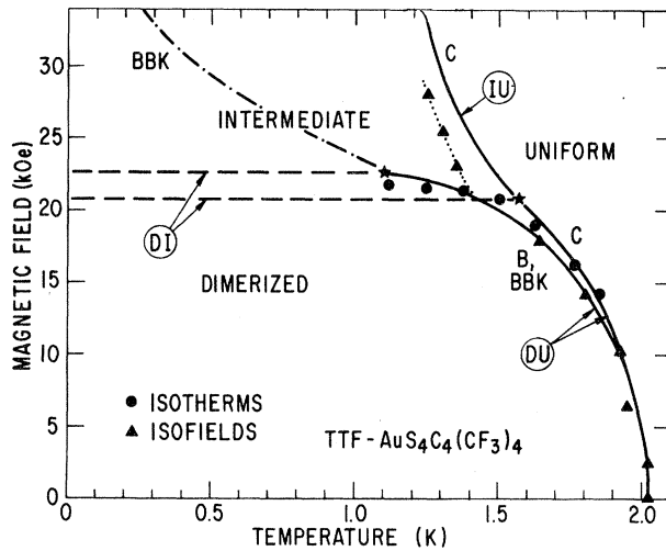
FIG. 3. Magnetic phase diagram for TTF-AuS 4 C 4 (CF 3 ) 4 , constructed from susceptibility maxima of Figs. 1 and 2. Theoretical curves of Cross (C), Bray (B), and Bulaevskii et al. (BBK) are shown along with their respective multicritical points (starred).
