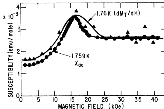
FIG. 5. Comparison of field dependence of differential susceptibility, \chi_{ac} , at 1.759 K with the isothermal susceptibility, (dM_T/dH) , obtained by differentiating the static magnetization data of 1.76 K.
