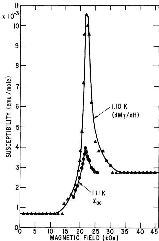
FIG. 6. Same as Fig. 5, for T \approx 1.1 K.
