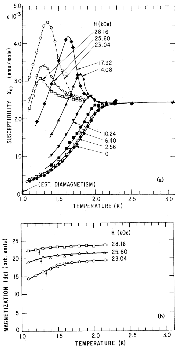
FIG. 1. (a) Differential susceptibility curves at various constant fields as a function of temperature for TTF-AuS 4 C 4 (CF 3 ) 4 . The curves for the special high-field region are shown as dashed lines. (b) Magnetization (static) curves as a function of temperature at several fixed fields for TTF-AuS 4 C 4 (CF 3 ) 4 . The arrows indicate the location of \chi_H(T) maxima from Fig. 1(a). The dotted curve shows the location of the singularity using a mean-field knee criterion.
