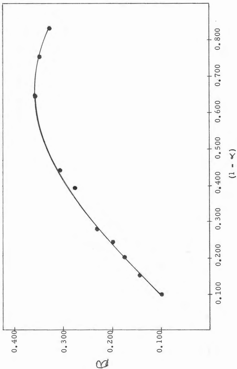
Figure 5. A plot of B versus (1 - \alpha) at a pH value of 6.9.
