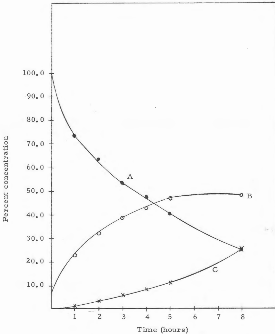
Figure 3. Concentration-time curves for substances A (hydrocortisone hemiester), B (hydrocortisone alcohol), and C (degradation products) at 70^{\circ}\text{C} . and a pH of 7.6.
