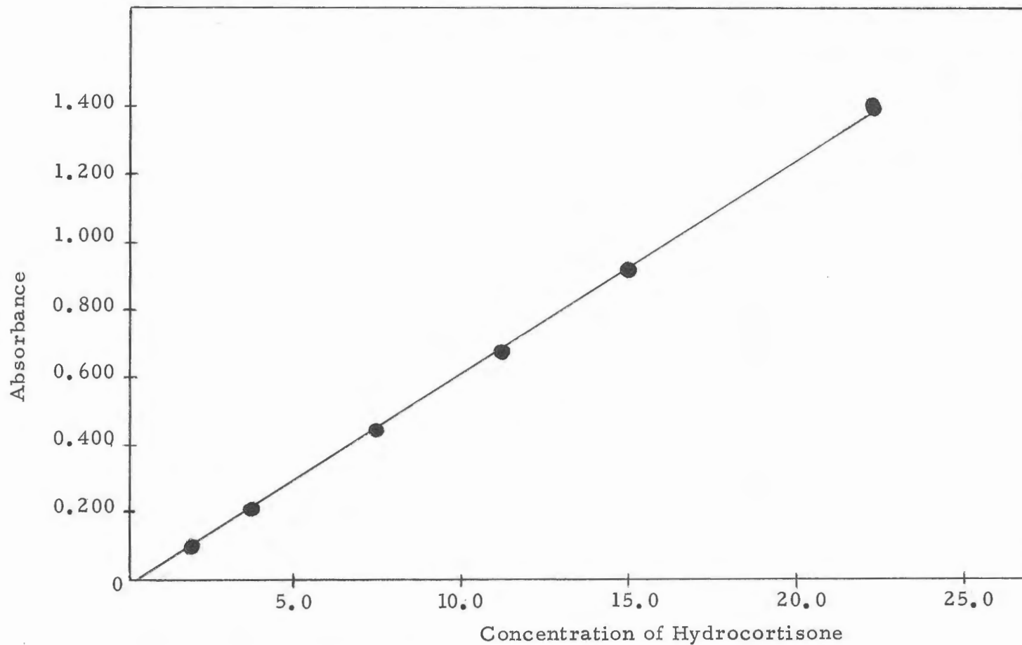
Figure A. A Beer-Lambert plot of absorbance versus the concentration of hydrocortisone (calculated as the free alcohol) in mcg./ml.
