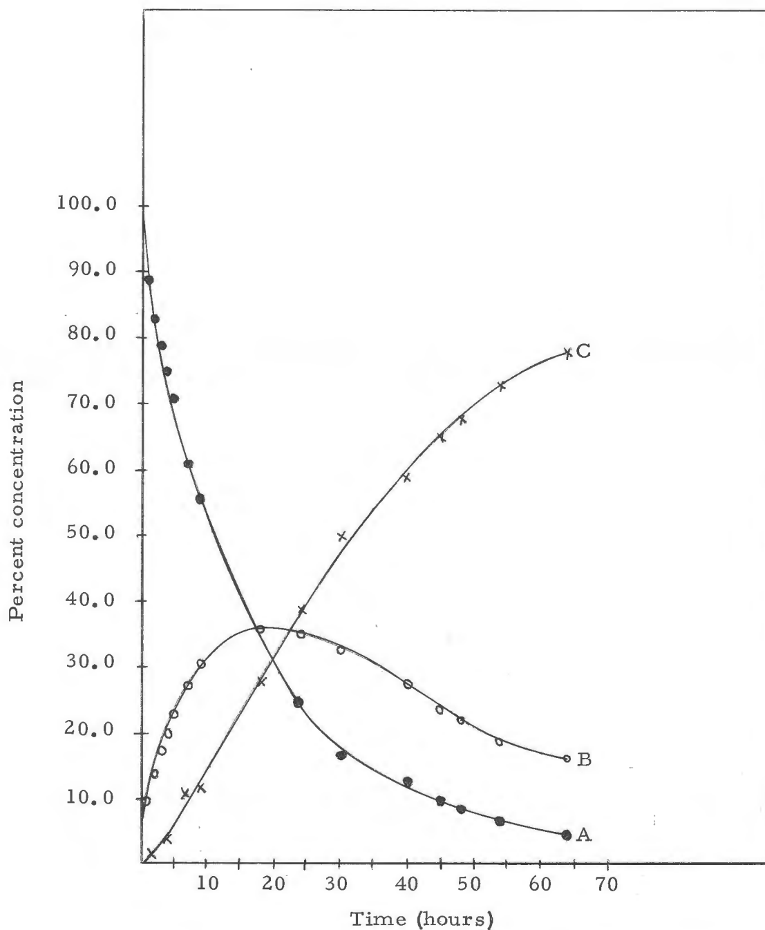
Figure 1. Concentration-time curves for substances A (hydrocortisone hemiester), B (hydrocortisone alcohol), and C (degradation products) at 70°C. and a pH of 6.9.
