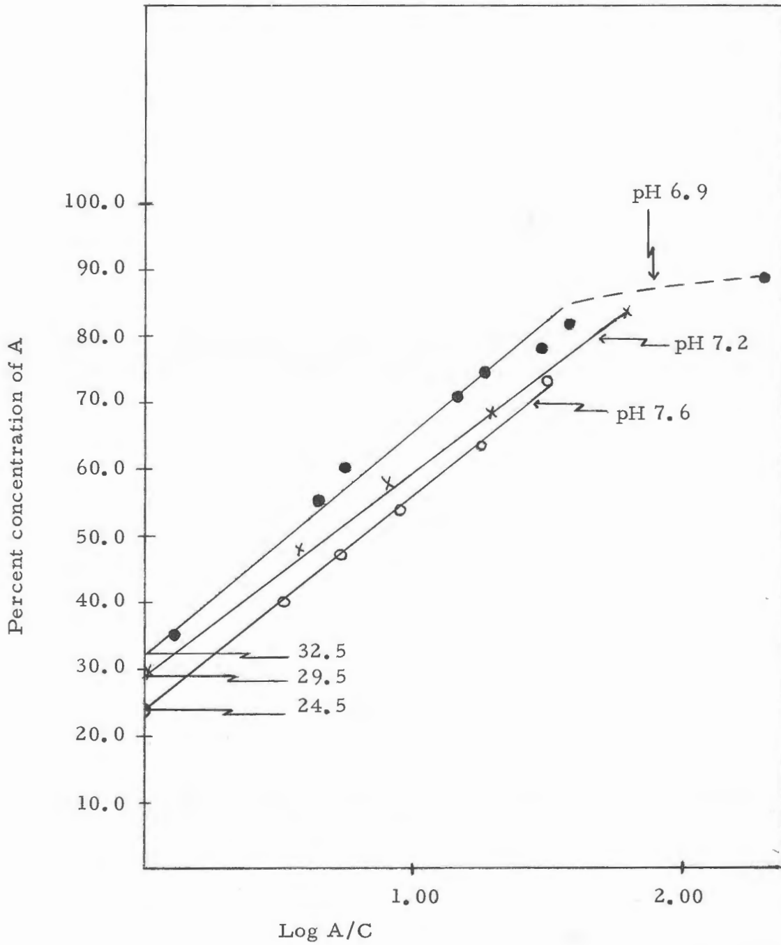
Figure 10. A plot of percent hydrocortisone sodium succinate (A) versus the log of the ratio of (A) and degradation products (C) for pH values of 6.9, 7.2 and 7.6.
