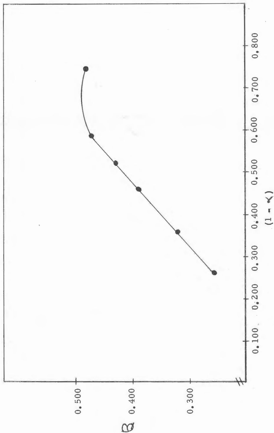
Figure 7. A plot of B versus (1 - \alpha) at a pH value of 7.6.
