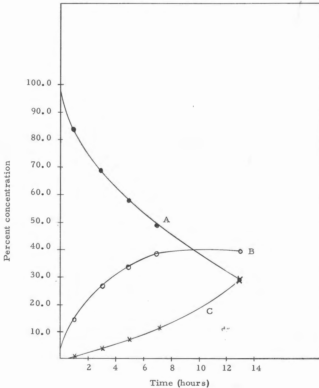
Figure 2. Concentration-time curves for substances A (hydrocortisone hemiester), B (hydrocortisone alcohol), and C (degradation products) at 70°C. and a pH of 7.2.
