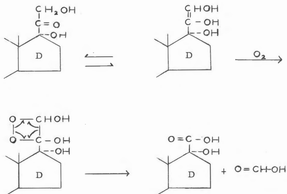
Proposed Degradation of the 17-Dihydroxyacetone Function in the Presence of Oxygen
