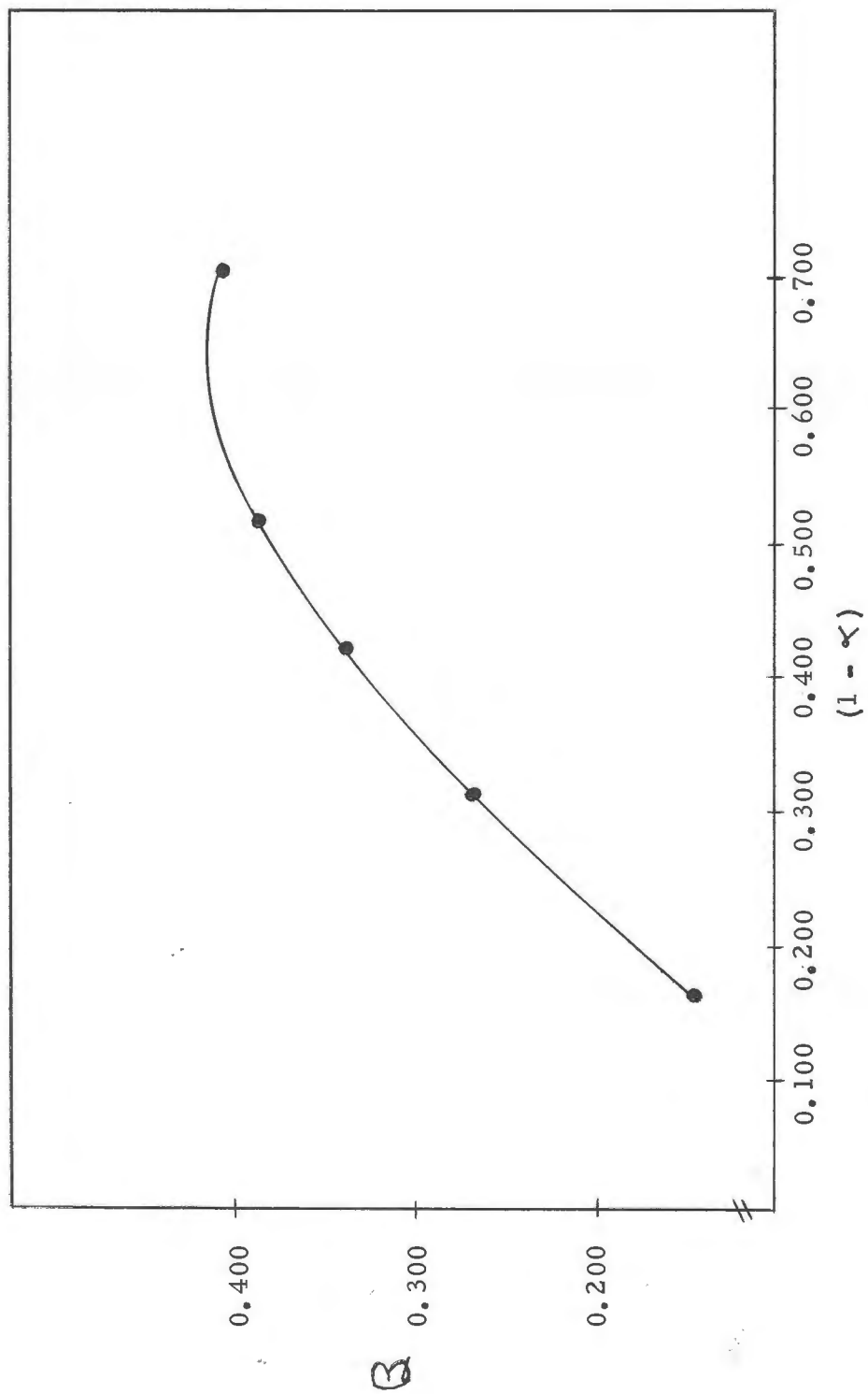
Figure. 6. A plot of B versus (1 - \alpha) at a pH value of 7.2.
