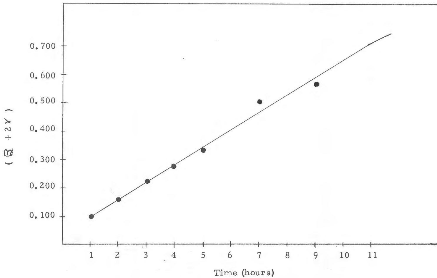
Figure 8. A plot of (B + 2Y) versus time at a pH value of 6.9.
