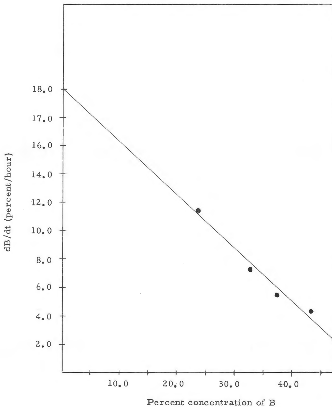
Figure 9. The rate of formation of hydrocortisone alcohol (dB/dt) versus the concentration of hydrocortisone alcohol (B) at 70°C, and a pH of 7.6.
