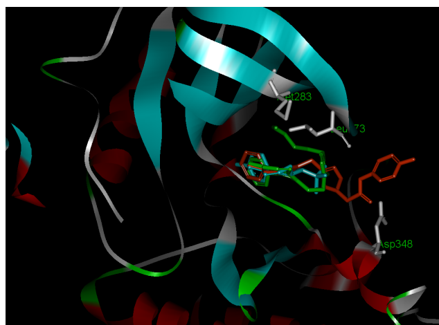
Figure 2. Comparison of structural complexes of Src kinase with different PhPP derivatives. 11b (green), PP1 (blue), and (b) 14f (red) based on molecular modeling. The compounds and side chains of amino acids are rendered in stick styles. Compounds are in the lowest energy conformers predicted. The Figure is drawn using the Accelrys visualization system.
