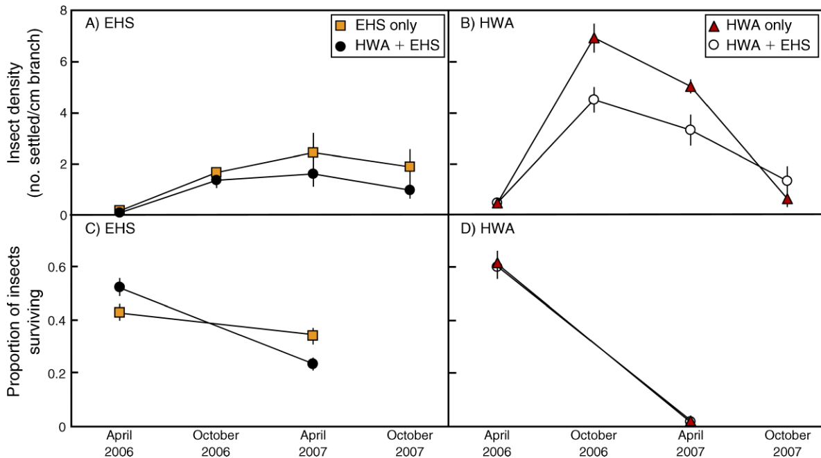
FIG. 1. Insect density and survival (mean \pm SE) over the winter period through the course of the experiment. (A) Fiorinia externa (EHS) density; (B) Adelges tsugae (HWA) density; (C) EHS survival in spring 2006 and 2007; (D) HWA survival in 2006 and 2007. Triangles, HWA-only treatment; squares, EHS-only treatment; solid circles, EHS density and survival in the HWA + EHS treatment; open circles, HWA density and survival in the HWA + EHS treatment.
