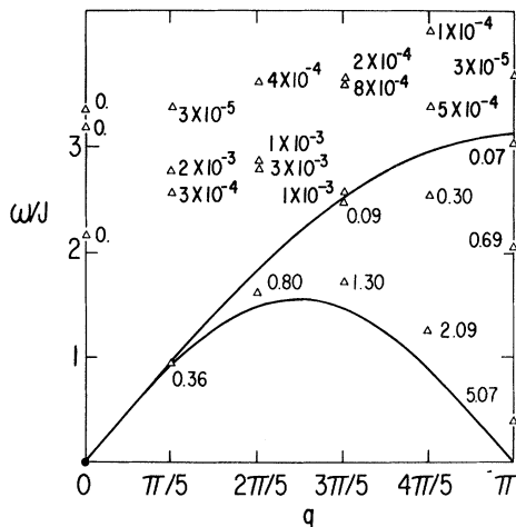
FIG. 1. G_{zz}(q, \omega) for a cyclic chain of N = 10 spins. For each q , G_{zz}(q, \omega) is a sum of \delta functions. The open triangles denote energy and wave number of the triplet excitations, and the numbers represent the corresponding spectral weight. At higher energies there are more triplets, not shown with very little spectral weight. No other excitations have nonzero matrix elements. The solid circle indicates the singlet ground state. The two solid lines represent E_1(q) and E_2(q) which form the lower and upper boundary of the SWDC in the thermodynamic limit.
