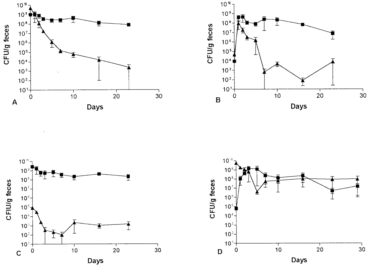
FIG. 4. Competitive mouse large intestine colonizing abilities. E. coli BJ4 (▲) and E. coli BJ4 rpoS (■) were fed simultaneously to four sets of three mice as follows: (A) both at 10^9 CFU; (B) both at 10^4 CFU; (C) BJ4 at 10^5 CFU and BJ4 rpoS at 10^9 CFU; (D) BJ4 at 10^9 CFU and BJ4 rpoS at 10^5 CFU. Error bars represent the standard errors of the geometric means.
