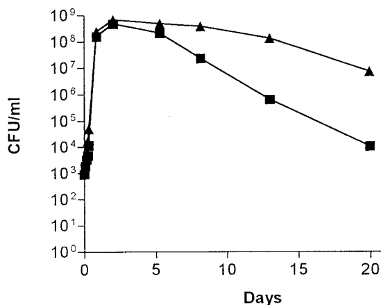
FIG. 1. Competitive growth and survival in minimal medium. E. coli BJ4 (▲) and E. coli BJ4 rpoS (■) were inoculated into minimal medium (0.2% glucose) and incubated with shaking (160 rpm) at 37°C for 20 days. Viable counts (CFU per milliliter) were determined at different time points by plating on selective medium.
