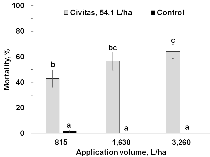
Figure 4. Effect of Civitas (54.1 L/ha) on mortality of Listronotus maculicollis adults at different carrier volumes. Means marked with the same letter do not differ statistically.
