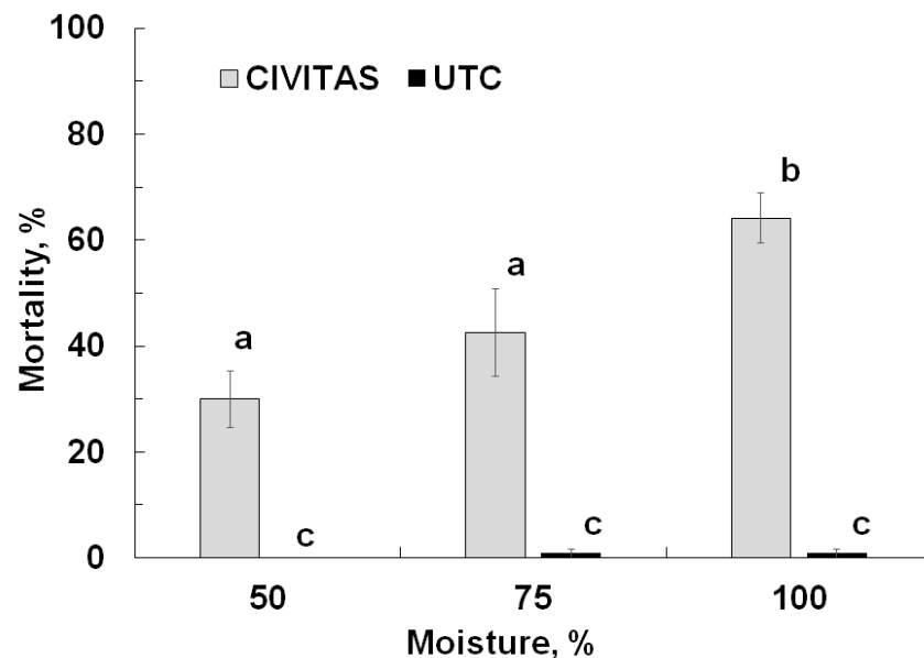
Figure 5. Mortality of Listronotus maculicollis (not corrected) adults caused by Civitas (54.1 L/ha) applied in 1630 L/ha carrier volume) at different soil moisture levels. Means marked with the same letter do not differ statistically.
