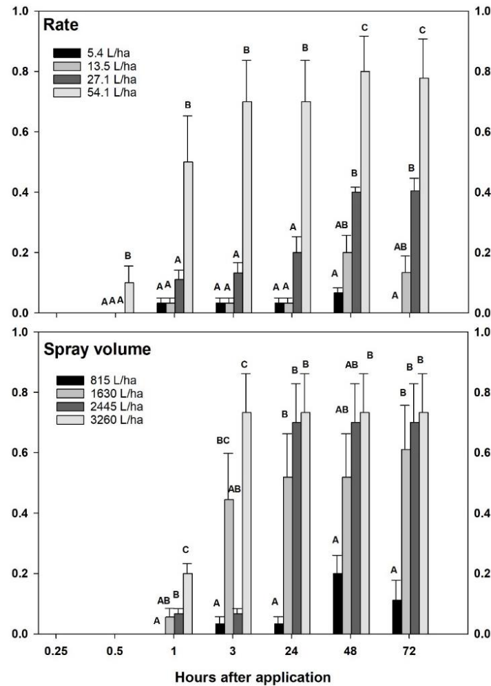
Figure 1. Cumulative effect of Civitas rate (top panel; at constant 815 L/ha carrier volume) and carrier volume (bottom panel; at constant 13.5 L/ha Civitas) on adult Listronotus maculicollis mortality between 0.25 to 72 h after application. Treatments within each interval were control corrected prior to analysis. Where polynomial contrasts detected significant relationships, one-way ANOVA was used to separate treatment means within time intervals at the \alpha = 0.05 . Means marked with the same letter do not differ significantly from one another.
