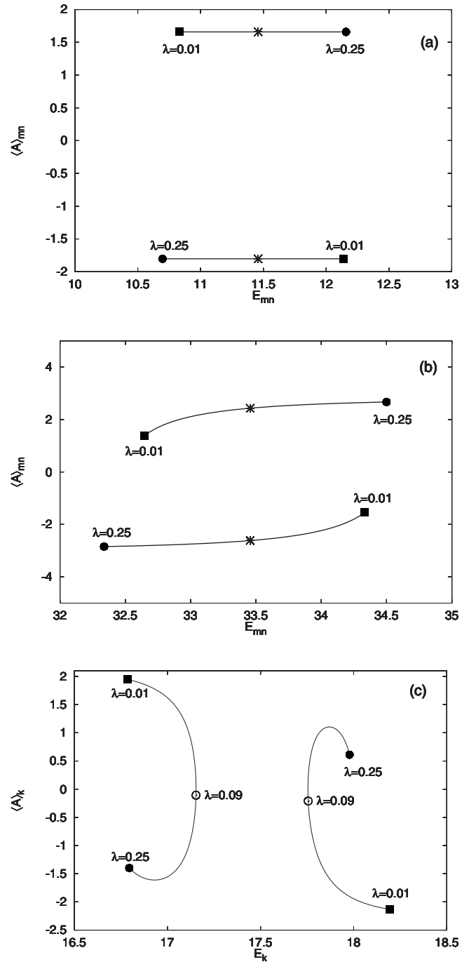
FIG. 3. Trace of one pair of eigenstates |\nu\rangle with parity P = +1 (identified by full circles in Fig. 2) in the plane of quantum invariants (E_{\nu}, \langle A \rangle_{\nu}) as the interaction parameter \lambda is increased a specified amount at constant value \alpha = (a) 0, (b) \pi/2 , and (c) \pi/4 of the integrability parameter. In the integrable regimes we use \nu = (m, n) and in the nonintegrable regime \nu = k .
