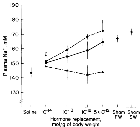
FIG. 5. Prevention of \text{Na}^+ loss from the plasma of hypophysectomized juvenile tilapia in fresh water by the 24-kDa PRL ( \bullet ) and the 20-kDa PRL ( \blacksquare ) but not by the 21-kDa GH ( \blacktriangle ). Both PRLs fully restore plasma \text{Na}^+ concentration from that found in saline-injected, hypophysectomized tilapia (Saline) to that found in sham-hypophysectomized tilapia in fresh water (Sham FW) or in sham-hypophysectomized tilapia acclimated to one-third strength seawater (Sham SW). n = 10 for each point except 5 \times 10^{-12} mol/g, where n = 3 .
