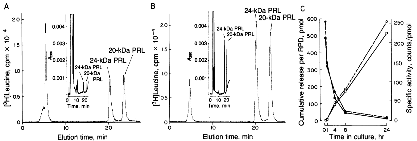
FIG. 4. Radiochromatographic analysis of secretory rates for the PRL pair in a [^3\text{H}] leucine pulse-chase experiment. (A) Reversed-phase HPLC of the medium collected after incubation of 13 PRDs after the 0.5- to 1-hr chase interval, indicating the elution of the proteins (Inset: absorbance at 280 nm) and elution of [^3\text{H}] leucine (5 min), the [^3\text{H}] leucine-labeled 24-kDa PRL (20 min), and the [^3\text{H}] leucine-labeled 20-kDa PRL (23 min). (B) Reversed-phase HPLC of the medium collected after incubation of 3 RPDs after the 4- to 8-hr chase interval. (C) Equal and constant release of both PRLs ( \circ , 24-kDa PRL; \square , 20-kDa PRL) during the 24-hr chase. Steady decline in specific activity ( \bullet , 24-kDa PRL; \blacksquare , 20-kDa PRL) of both PRLs in the medium indicates an interval of <1.5 hr between synthesis and release in these culture conditions.
