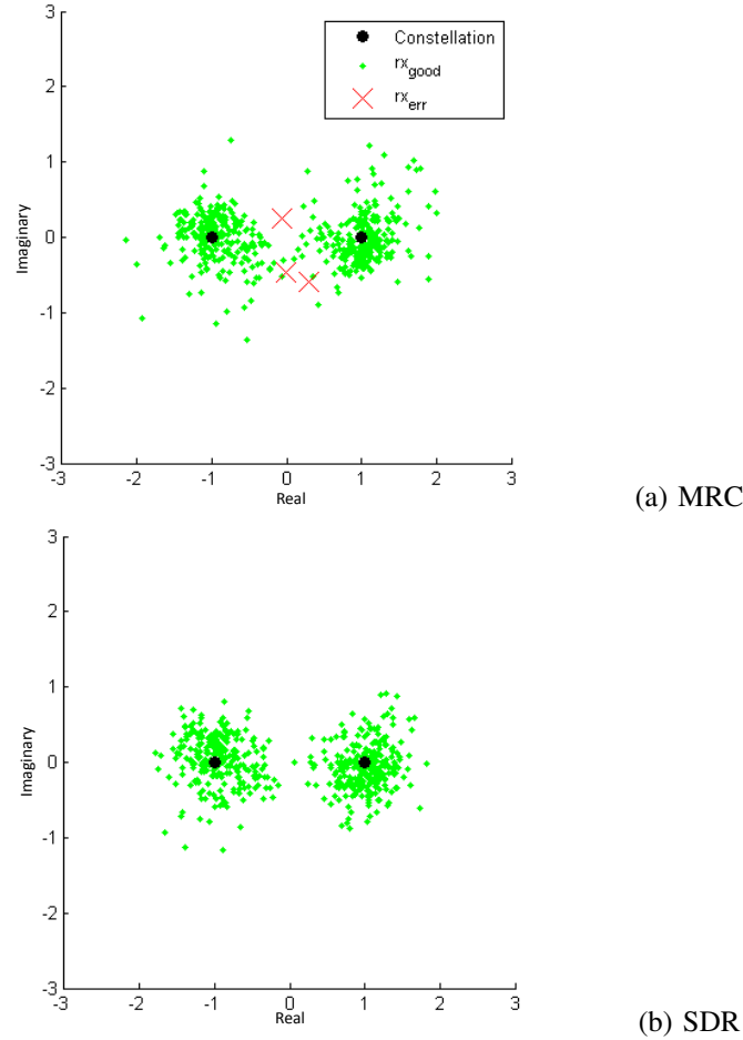
Figure 8. Received symbol constellations obtained using Maximum Ratio Combining (panel a) and Spatial Diversity Reconstruction (panel b).
