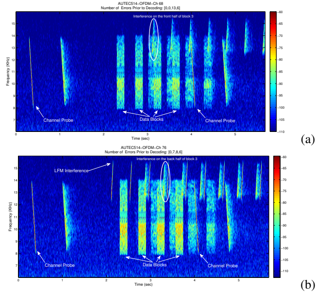
Figure 7. The OFDM signals received on channels 68 (panel a) and 76 (panel b) during an experiment at AUTEc in May 2014. Note that LFM interference corrupts for the beginning of block 3 of the data packet on channel 68 and the end of the same block on channel 76.
