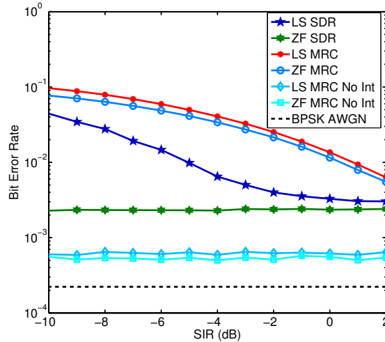
Figure 6. Bit Error Rate for different combining strategies and equalization methods at an SNR of 7.9 dB and various SIRs: SDR - Spatial Diversity Reconstruction, MRC - Maximum Ratio Combining, No Int - No interference present, LS - Least Squares Equalizer, ZF - Zero Forcing Equalizer, BPSK AWGN - binary phase shift keying on an impulse channel in additive white Gaussian noise.
