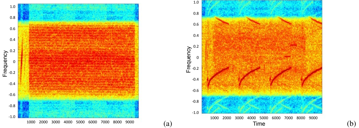
Figure 2. Clean packet reception (a) and packet corrupted by acoustic interference (b).
