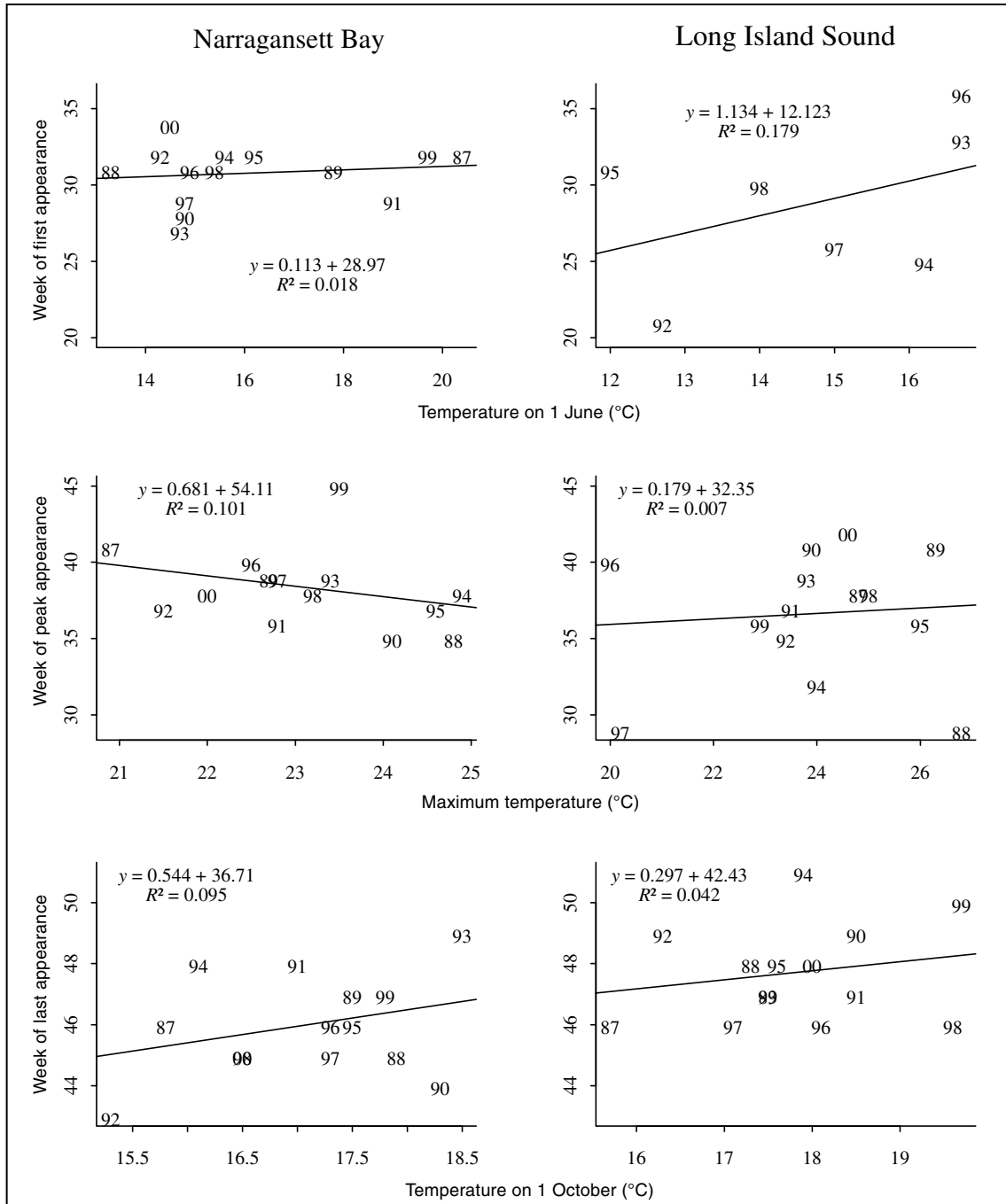
Figure 7 Correlations between temperatures and weeks of the year (1–52) of first (5% of peak), last, and peak appearance of warm-water fishes in both Narragansett Bay and Long Island Sound (1987–2000).
