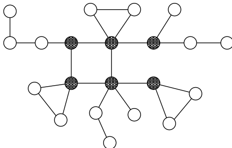
Figure 4: A graph in \mathcal{S}_6
