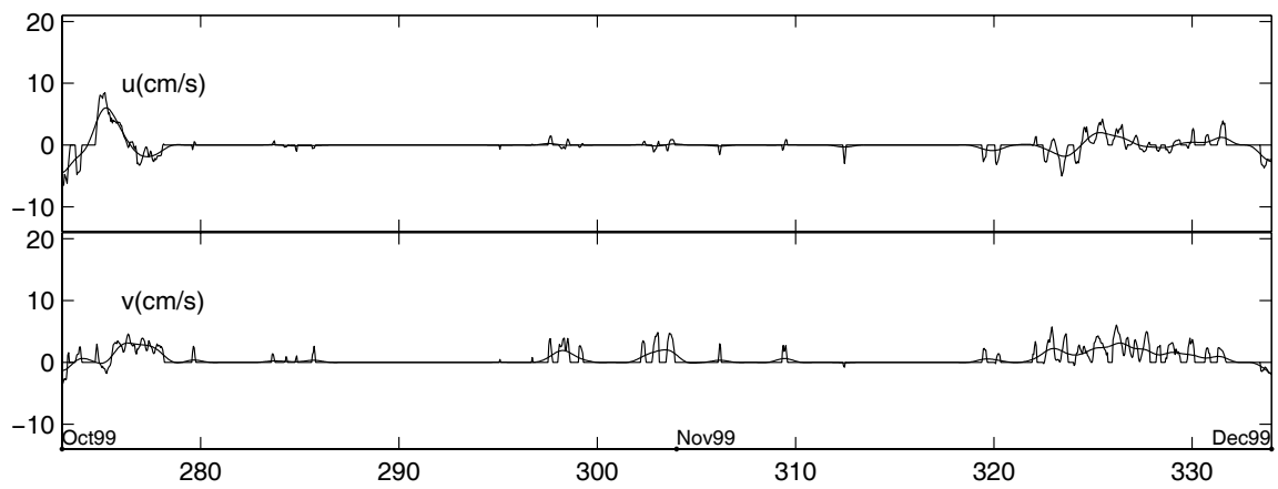
Figure 7: M1-3 Hourly and 40 HRLP Velocities
