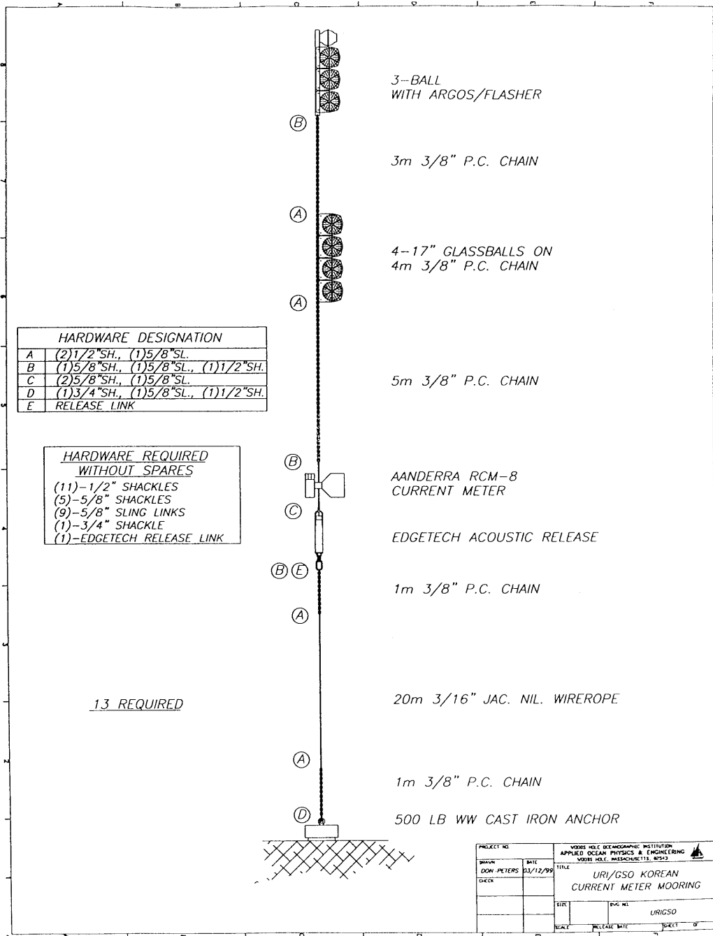
Figure 2: Schematic of the mooring designs of the Aanderra current meter. Glass balls and 500 lb anchor were used to hold the mooring line taut.
