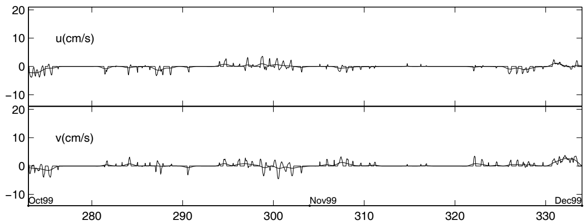
Figure 8: M1-5 Hourly and 40 HRLP Velocities
