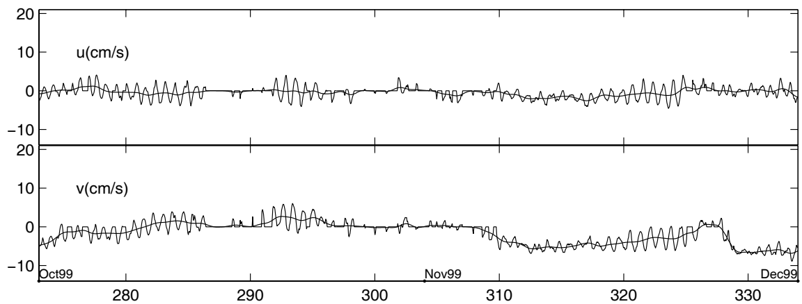
Figure 11: M3-1 Hourly and 40 HRLP Velocities
