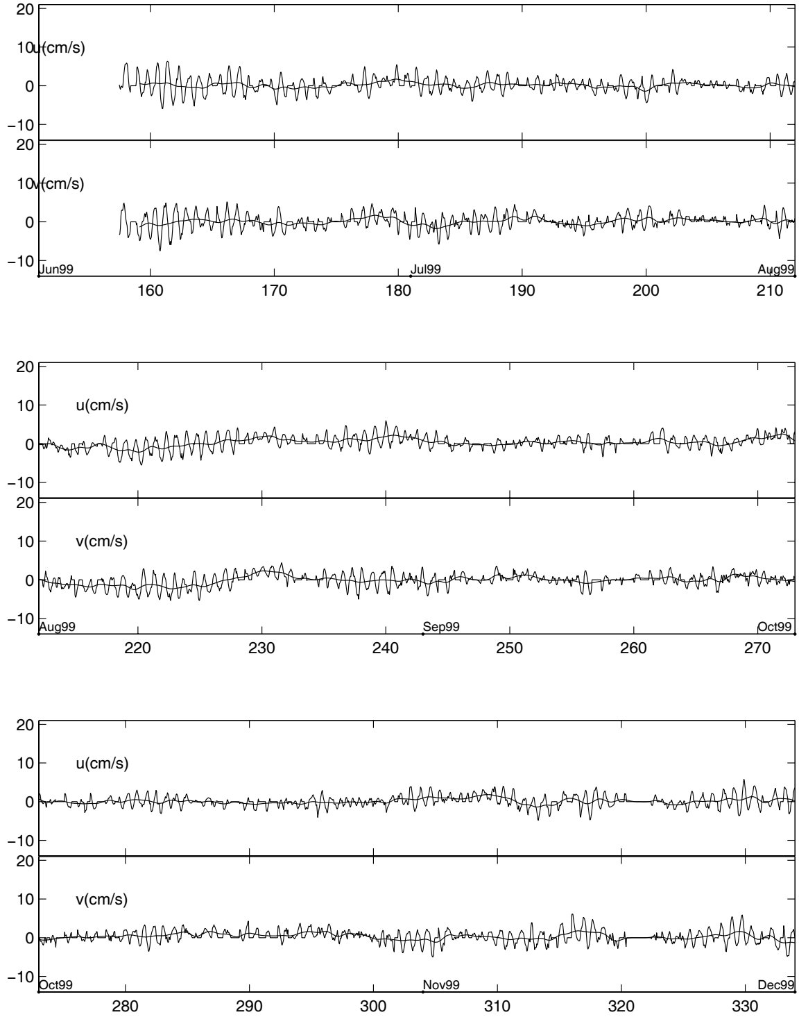
Figure 13: M4-1 Hourly and 40 HRLP Velocities
