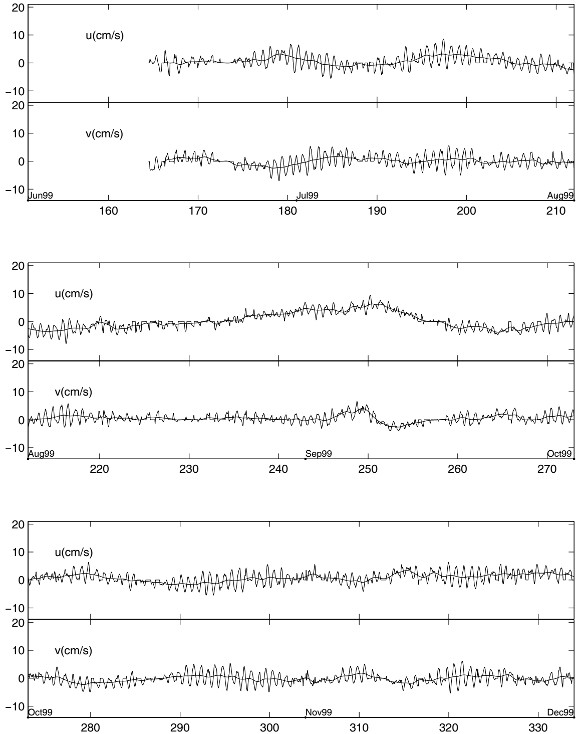
Figure 14: M4-3n Hourly and 40 HRLP Velocities
