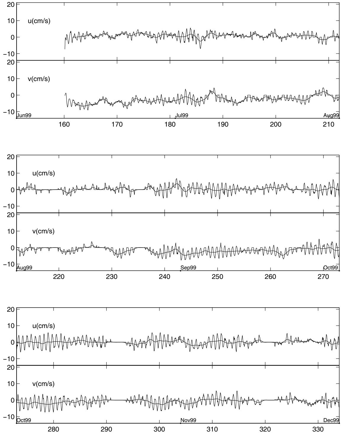
Figure 5: M1-1 Hourly and 40 HRLP Velocities
