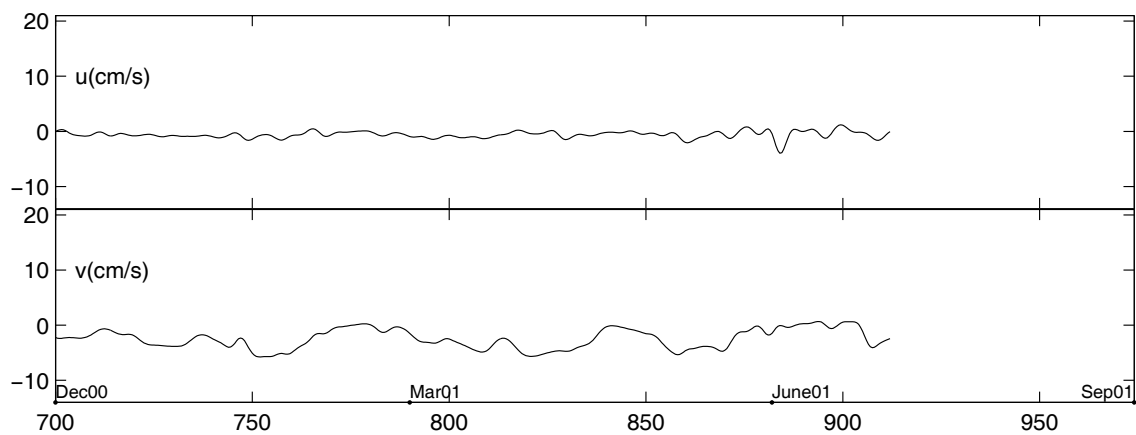
Figure 22: M3-1 120 HRLP Velocities
