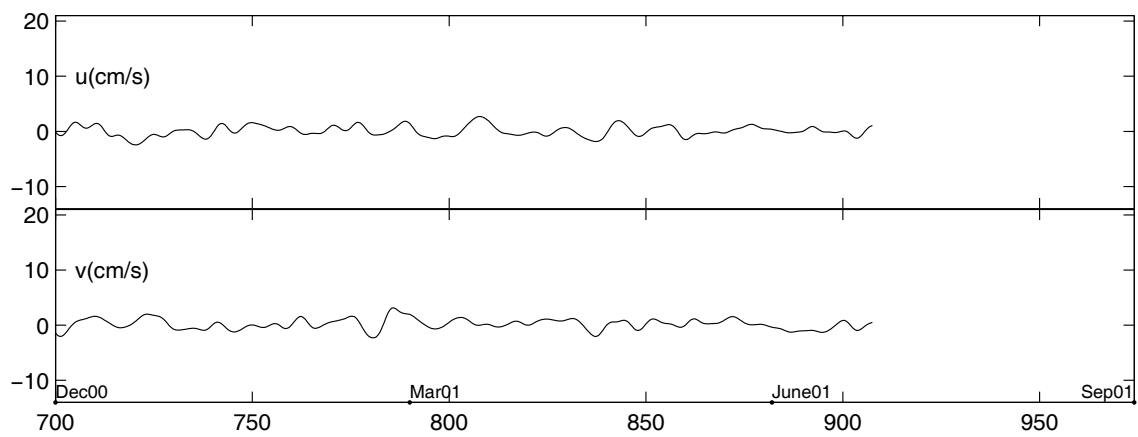
Figure 24: M4-1 120 HRLP Velocities
