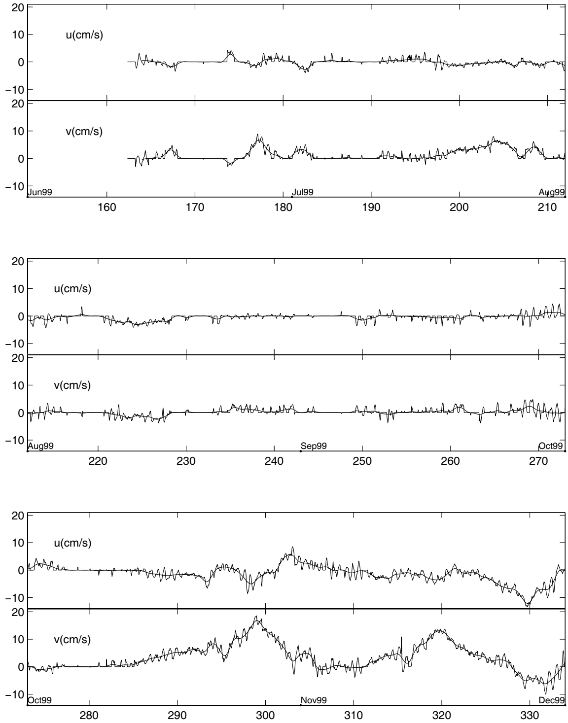
Figure 9: M2-1 Hourly and 40 HRLP Velocities
