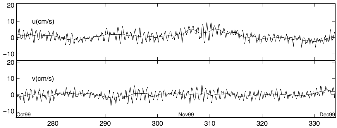
Figure 15: M 4-3s Hourly and 40 HRLP Velocities
