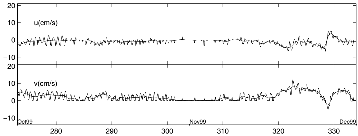
Figure 6: M1-2 Hourly and 40 HRLP Velocities
