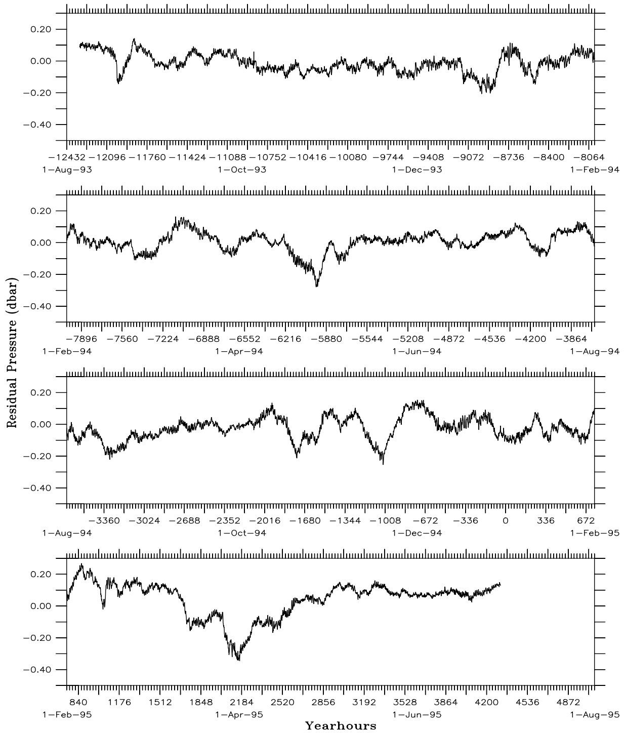
Figure 18: PIES95NAC65 Residual Pressure Record
