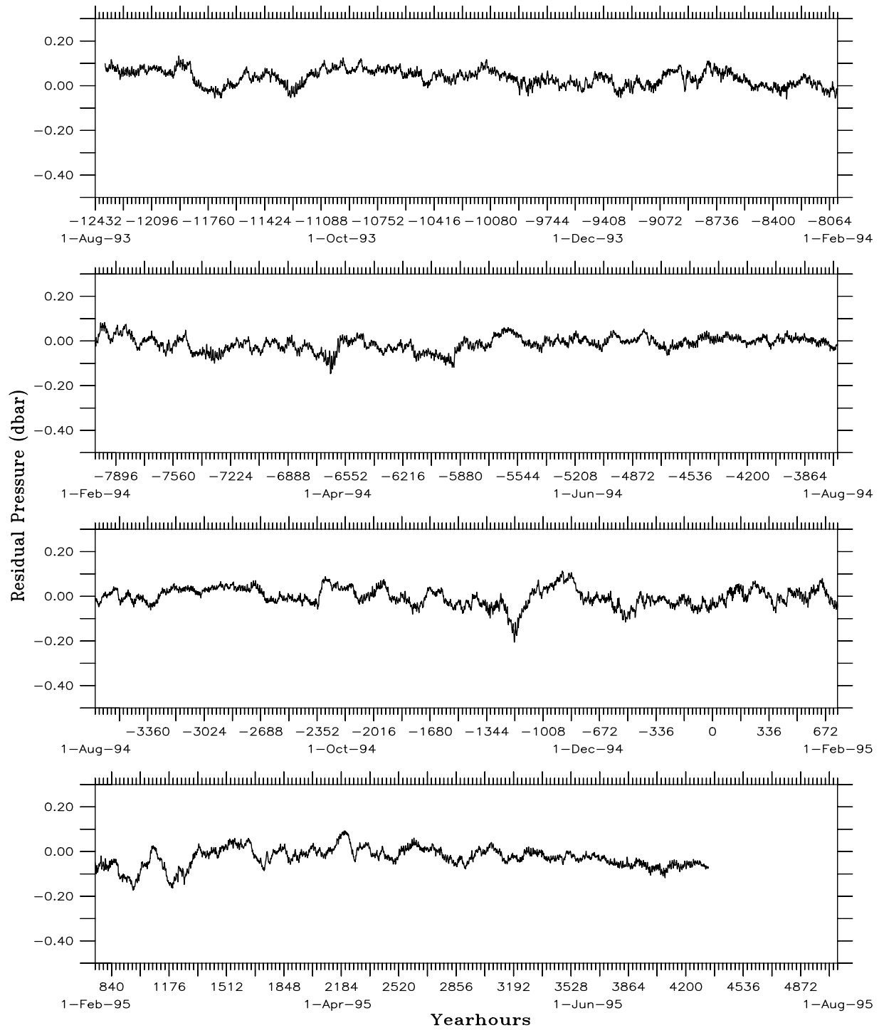
Figure 17: PIES95NAC40 Residual Pressure Record
