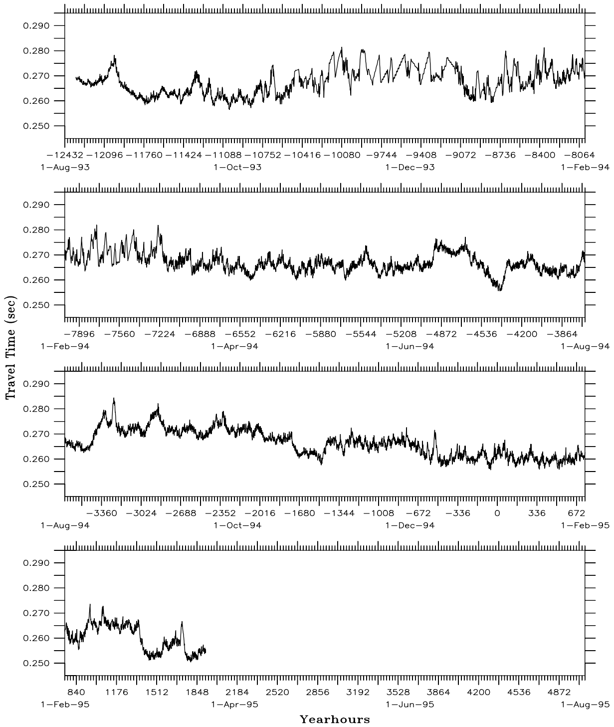
Figure 10: PIES95NAC65 Travel Time Record
