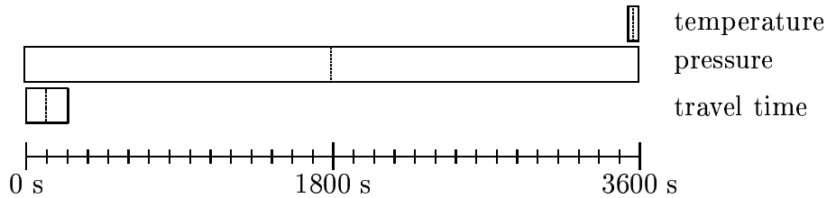
Figure 3: Sampling Sequence of Sea Data Model PIESs. The horizontal length and position of the boxes represent the duration and relative timing of the measurements of travel time, pressure, and temperature during each sampling period. The midtime of each variable is indicated by a dotted line. Tick marks represent 2 minute intervals.
