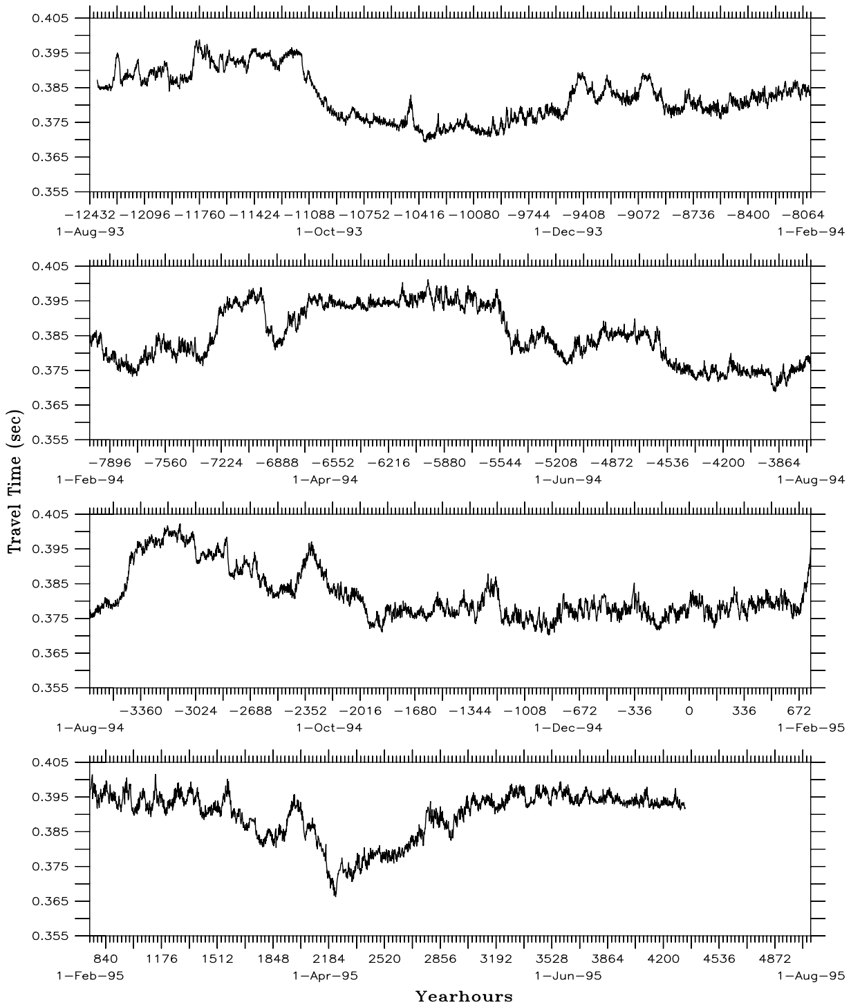
Figure 9: PIES95NAC40 Travel Time Record
