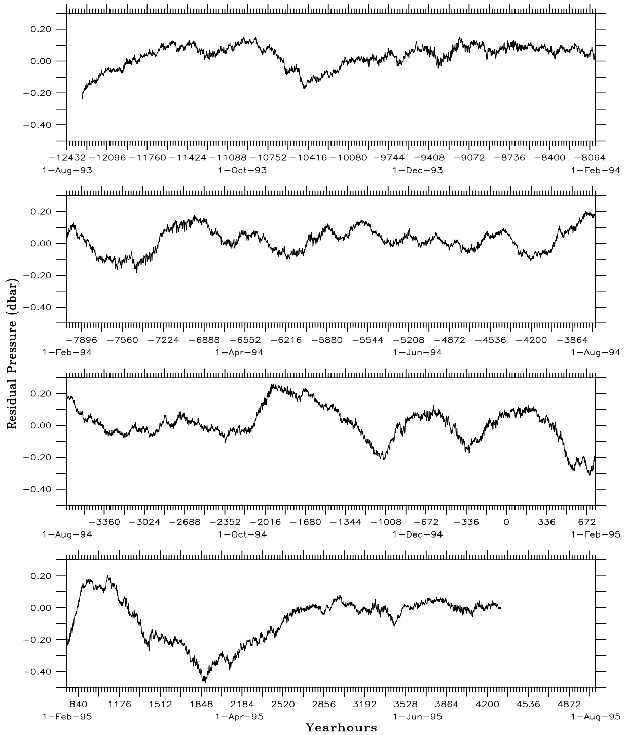
Figure 19: PIES95NAC80 Residual Pressure Record
