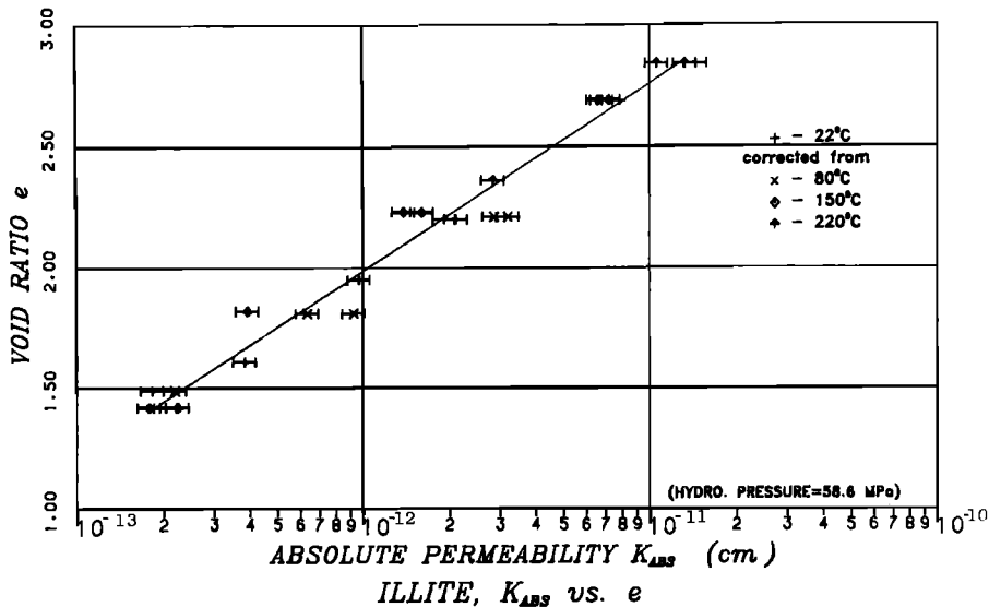
Fig. 9. Absolute permeability (corrected for temperature) versus void ratio for illite. Hydrostatic pressure is constant at 58.6 MPa. K_{abs} = 101.30e - 14.57 cm 2
