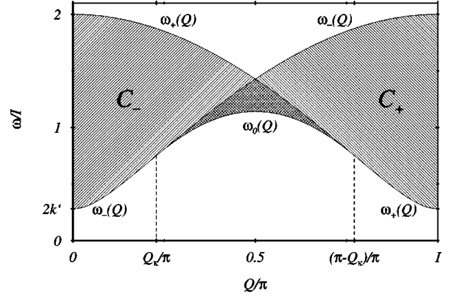
FIG. 1. Two-spinon excitation spectrum (3.1) for k=0.99 ( \Delta \approx -2.305 ). It consists of two partly overlapping sheets C_- and C_+ . Sheet C_+ lies between \omega_0(Q) and \omega_-(Q) in the range Q_\kappa \leq Q \leq \pi - Q_\kappa and between \omega_+(Q) and \omega_-(Q) for \pi - Q_\kappa \leq Q \leq \pi . Sheet C_- is obtained from C_+ by reflection about the line Q = \pi/2 . The interval (0, \pi) represents one-half of the extended Brillouin zone, in which one ground-state vector |0\rangle is assigned the wave number Q=0 and the other ground-state vector |\pi\rangle the wave number Q=\pi .
