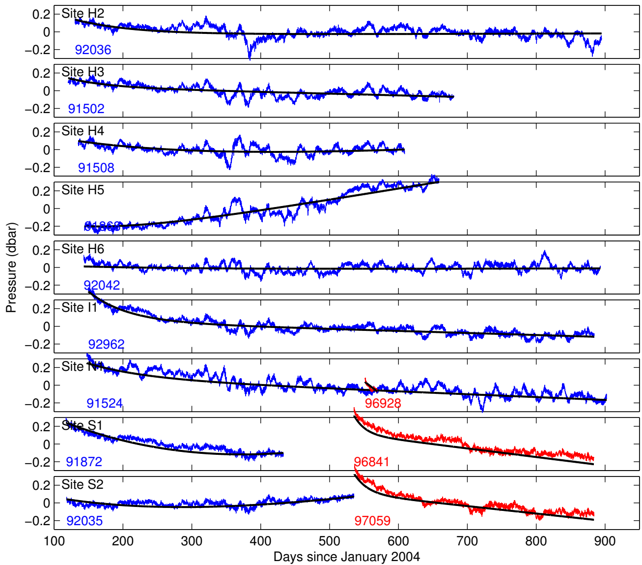
Figure 18: Time series of hourly pressure with drift curves superimposed (lines H-S). The Paroscintific pressure sensor SN is shown below the beginning of the time series.
